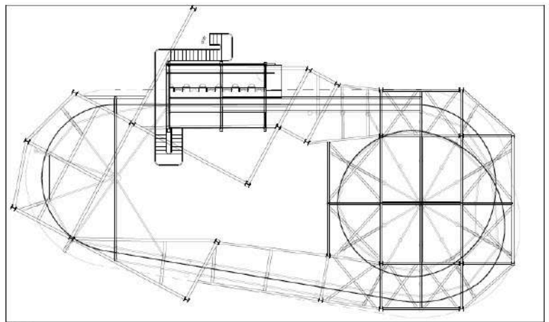
— FORCE ONE COASTER — 1 : 100
